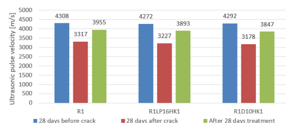
Figure 5. UPV in three states measured longitudinally.
