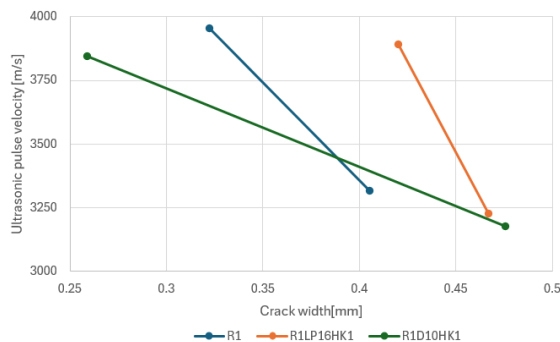
Figure 7. Correlation of UPV in longitudinal direction with the crack width before and after treatment.
