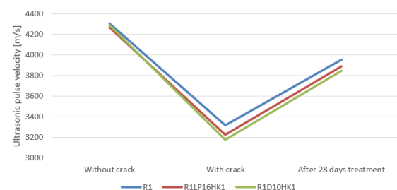
Figure 6. UPV in three states measured longitudinally.
