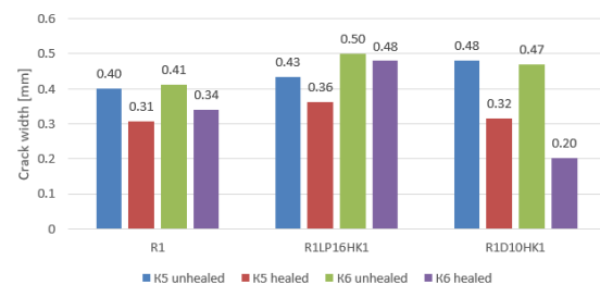
Figure 8. Measured crack width before and after treatment.
