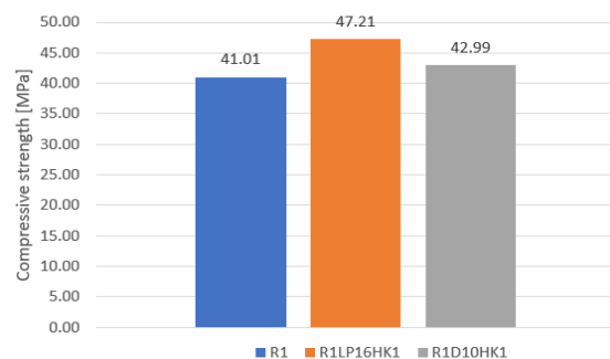
Figure 3. Compressive strength of specimens.
