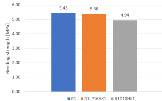
Figure 4. Bending strength of specimen.
