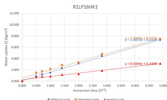
Figure 9. Capillary absorption of samples from R1LP16HK1 mix design.
