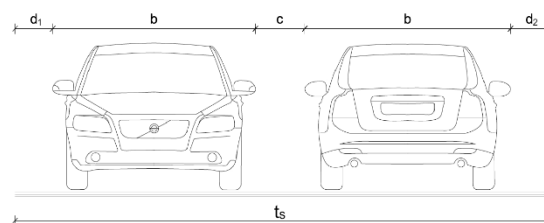
Figure 1. Carriageway width
