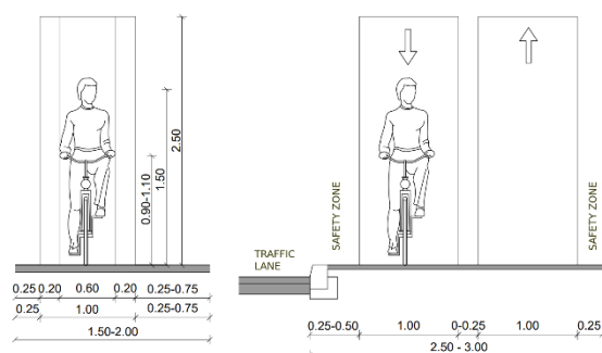
Figure 3. Cycling path, lane width
