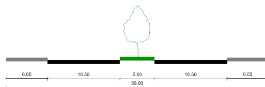
Figure 4. Cross-section of the boulevard according to the City of Skopje GUP 2012-2022
