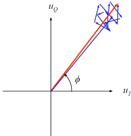
Fig 2. Representation of a Permanent Scatterer within the resolution cell [5]
