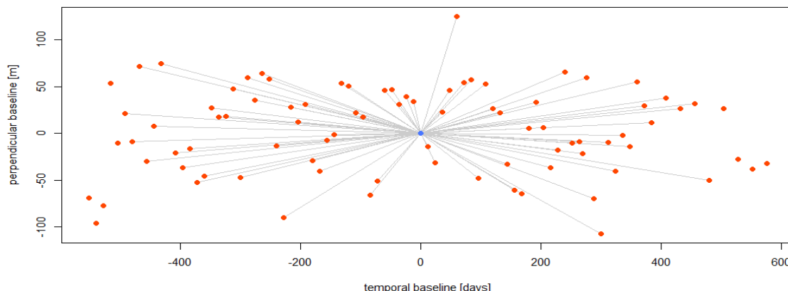
Fig.7 PSInSAR graph of the connection between the reference and secondary images.
