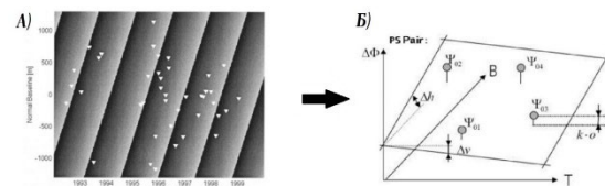
Fig. 5 A) Periodogram showing the spatial-temporal dependence; B) Best-fitting 2D plane, whose slopes represent the linear values of the PS pair. [3]
