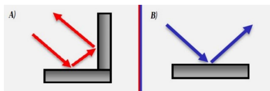
Fig 3. A) Dihedral Scattering B) Specular Scattering
