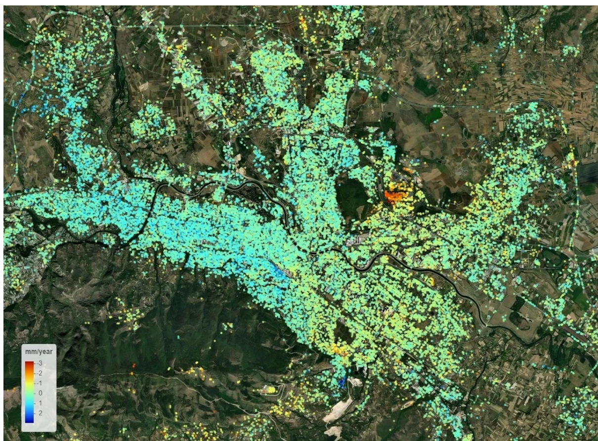
Fig.8 Deformation Results from the Conducted PSInSAR Analysis for the Skopje Basin Displayed in the STaMPS Visualizer Software
