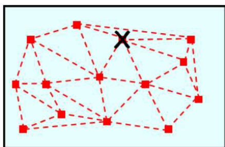
Fig. 6 PS network integration [6]
