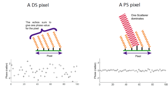
Fig 4. Representation of phase variation in PS and DS pixels. [5]
