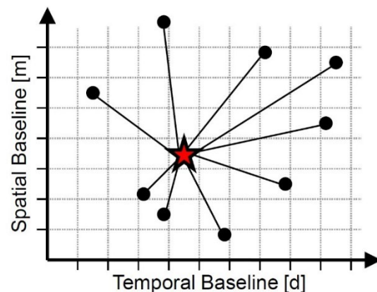
Fig 1. Schematic representation of interferogram generation in PSInSAR. [1]
