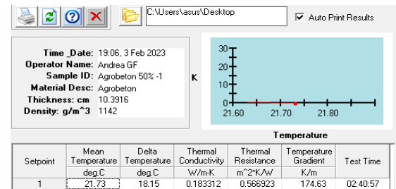
Figure 8. Results for the sample with 50% straw
