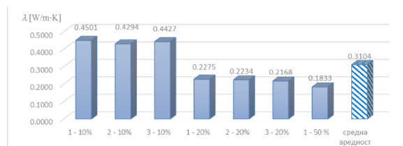
Figure 9. Thermal conductivity for all tested samples
