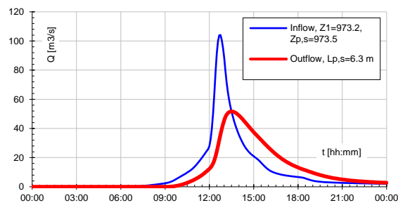
Figure 8. Hydrograph of flood wave for Petrova river, with recurrence interval of T = 10\,000 years, inflow and outflow hydrograph
