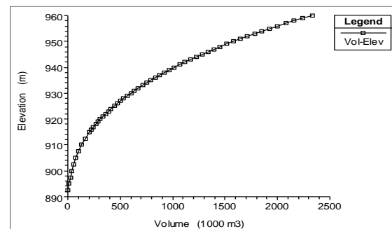
Figure 6. Volume – elevation curve for Sasa 4 TSF
