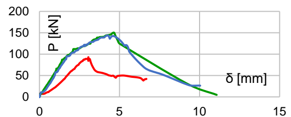
Figure 6. P-δ diagram for anchor type 1
