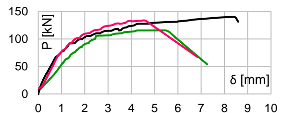
Figure 7. P-δ diagram for anchor type 2
