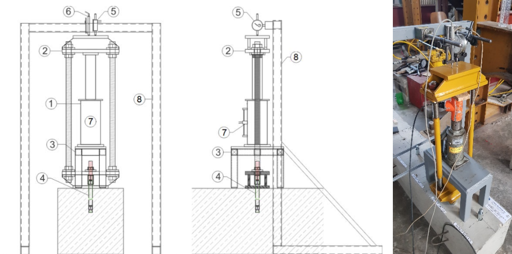
Figure 5. Scheme for installation of the equipment
