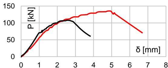
Figure 13. P- \delta diagram for anchor type 8
