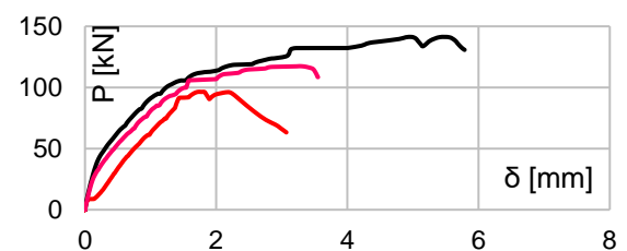
Figure 8. P-δ diagram for anchor type 3
