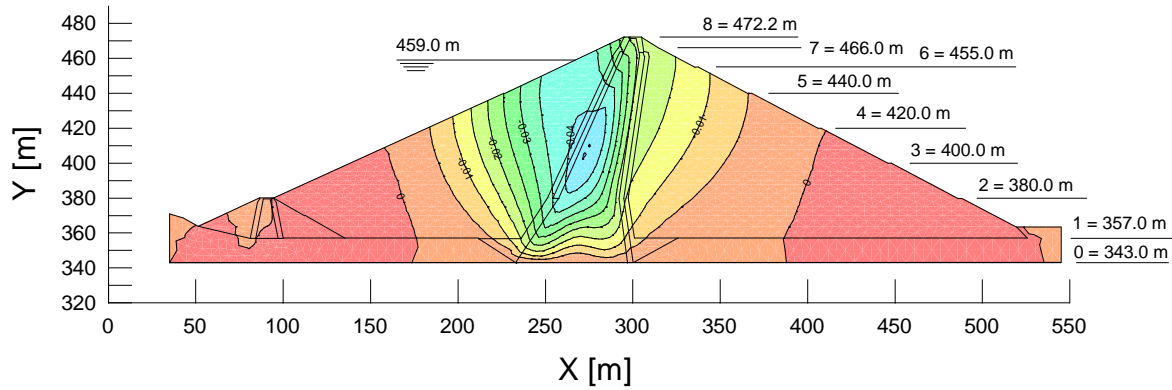
Figure 7. State upon consolidation, dY displacement (-0.045) - (+0.001) m
