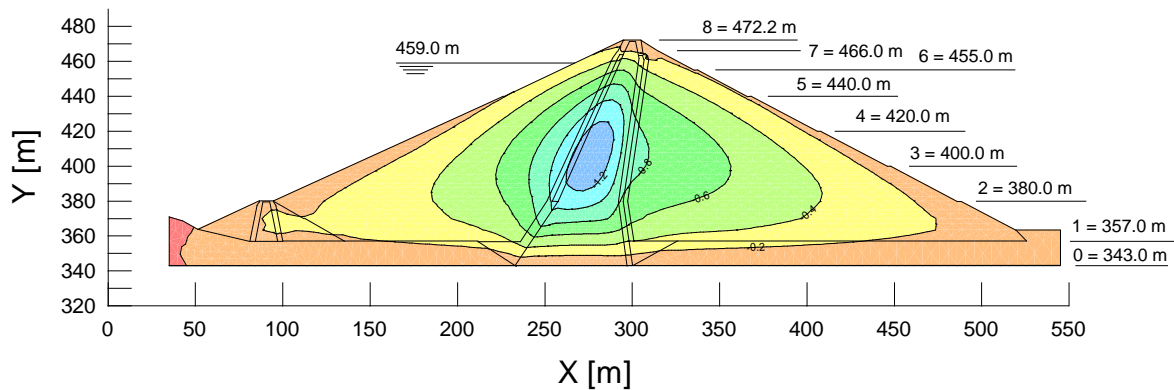
Figure 5. State after dam construction, Ydisplacement (-1.338) - (+0.012) m
